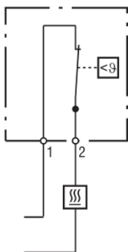
Thermostat
