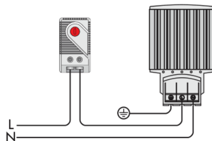
Thermostat
